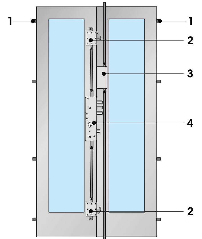
Vitra a Cilindro D.B. pred. Vetro Camera
