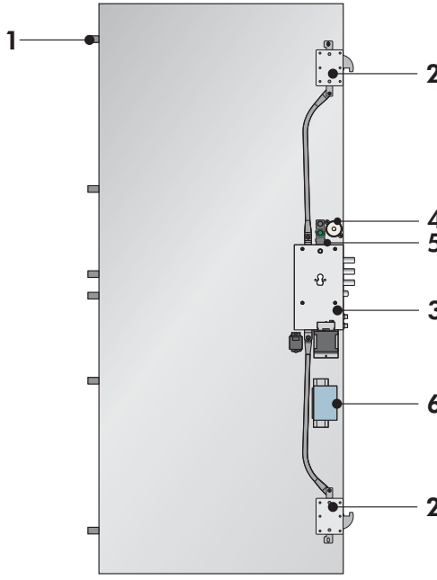
Synergy Out Next Elettra
