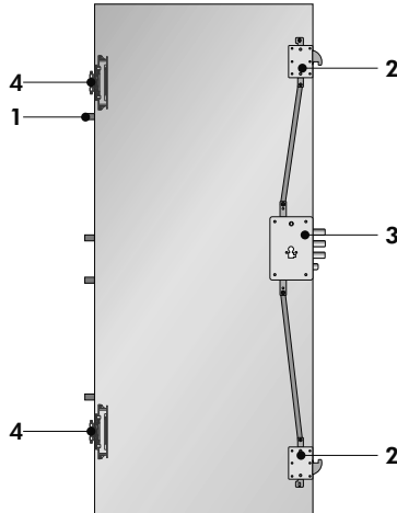
Sleek Sentry1 Standard e legno avvolgente - Standard and enveloping wood
