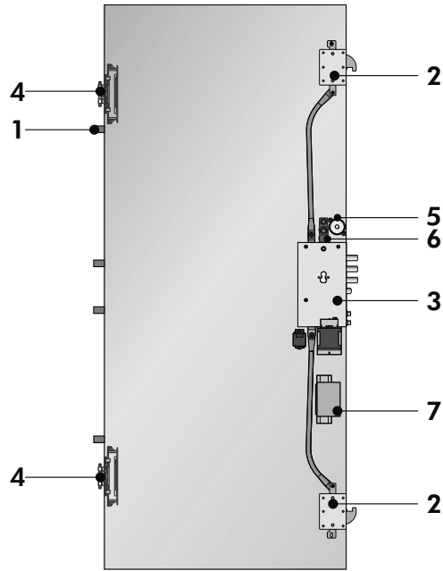
SleekOut Next Elettra
