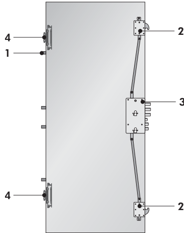
Sleek Sentry Doble Standard e legno avvolgente - Standard and enveloping wood
