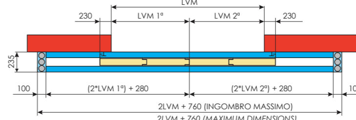
CON PORTINA PEDONALE WITH PEDESTRIAN DOOR
